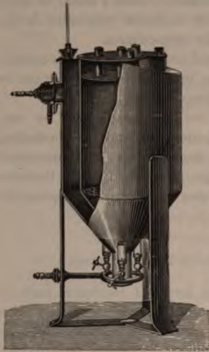
FIG. 16.—D'ARSONVAL'S INCUBATOR.
